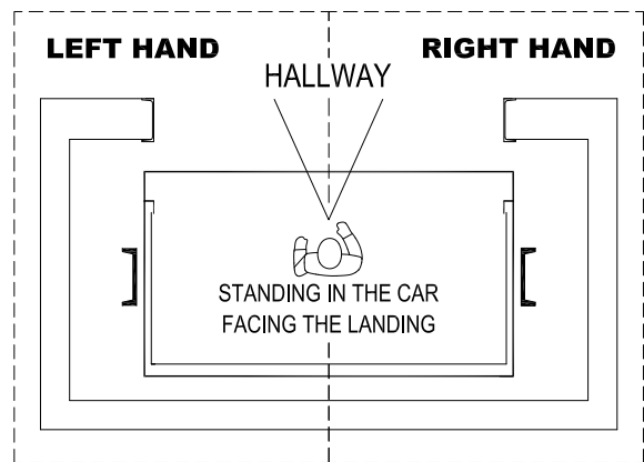
PLAN VIEW OF HOISTWAY
