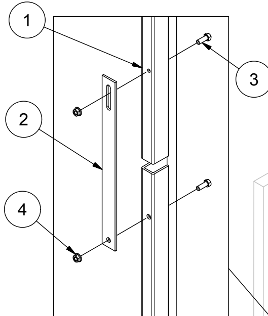
0354 Mechanical Lock (option)
