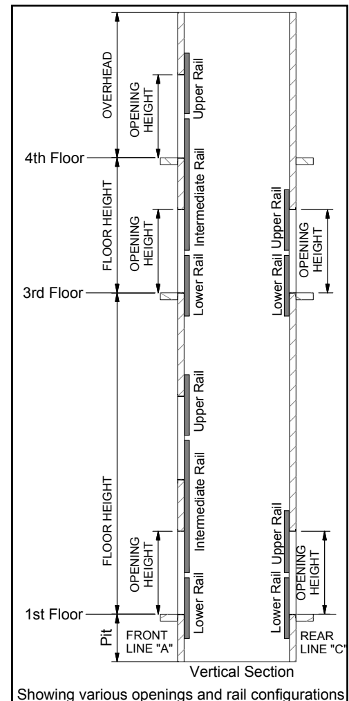
Figure 2 - Door Rail Categories
