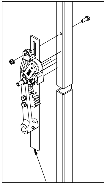
0354 Mechanical Lock (option)
