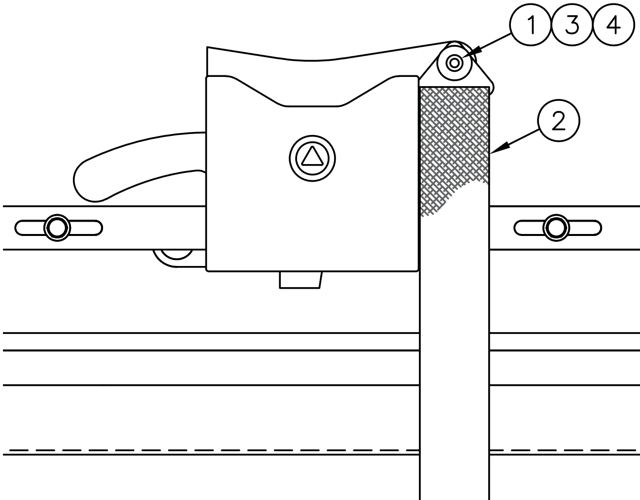
VIEW FROM HOISTWAY (BACK OF DOOR PANEL)
