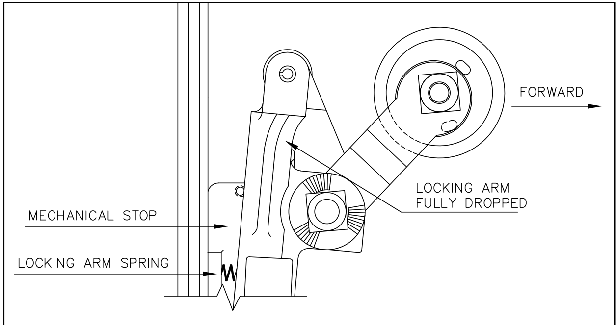
Figure 6 - Roller Arm Setting
