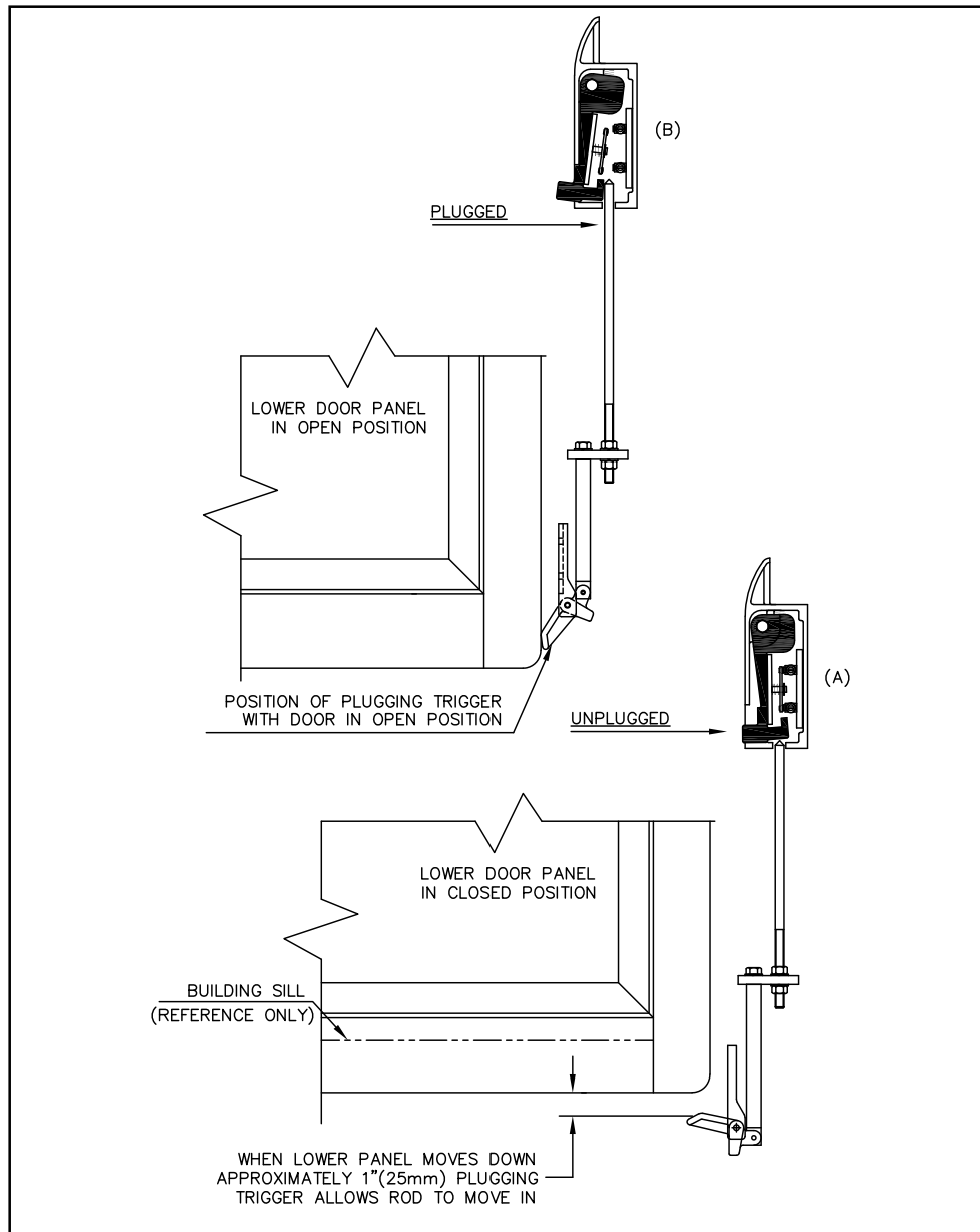
Figure 4 - Plugging Trigger
