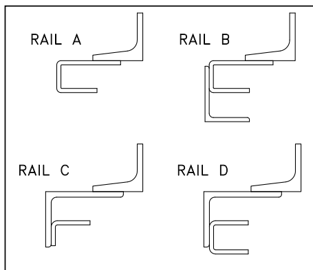
Figure 1 - Door Rail Types
