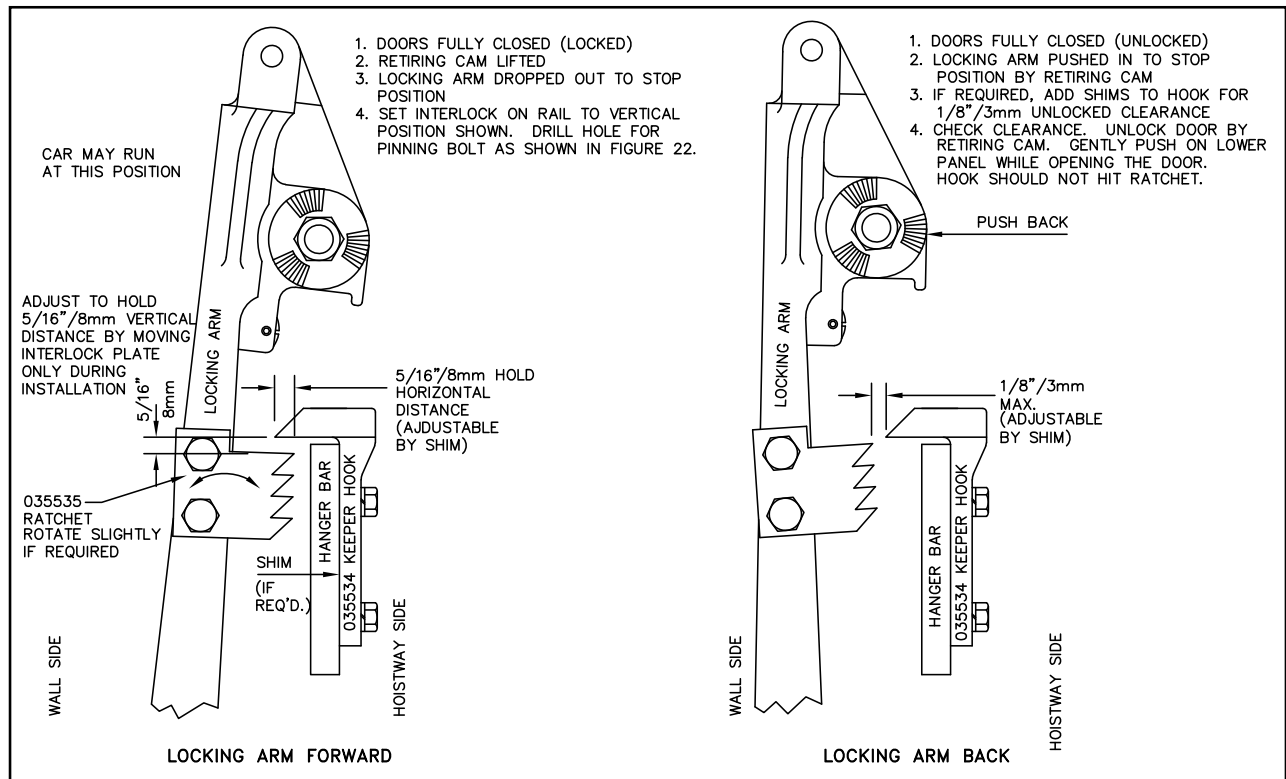
Figure 5 - Locking Arm
