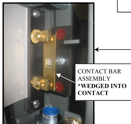
RETAINING RING DISLODGED (PROBLEM CONDITION)
