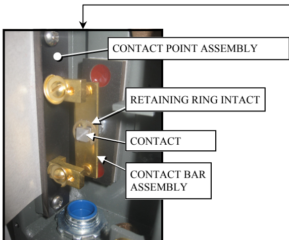
RETAINING RING INTACT (NORMAL CONDITION)
