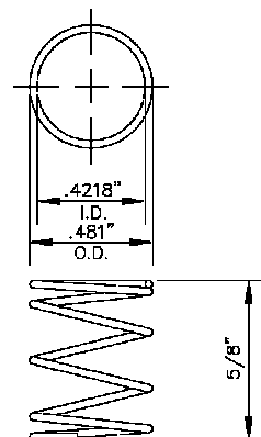
033171 CONTACT SPRING
