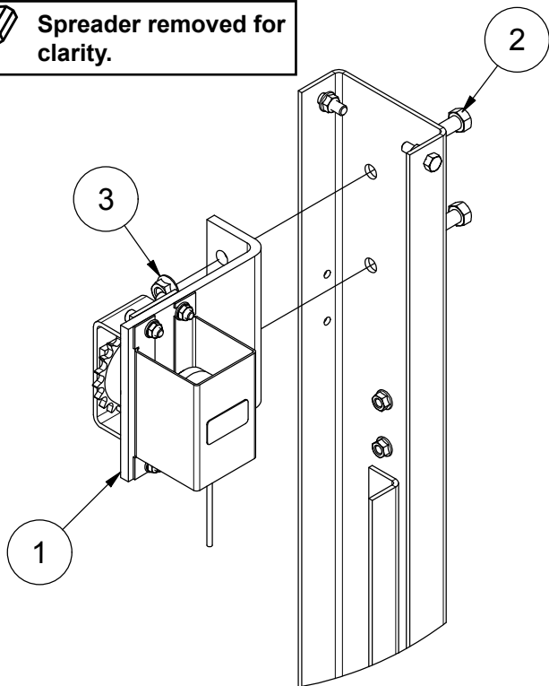
DETAIL A IDLER & ENCODER
