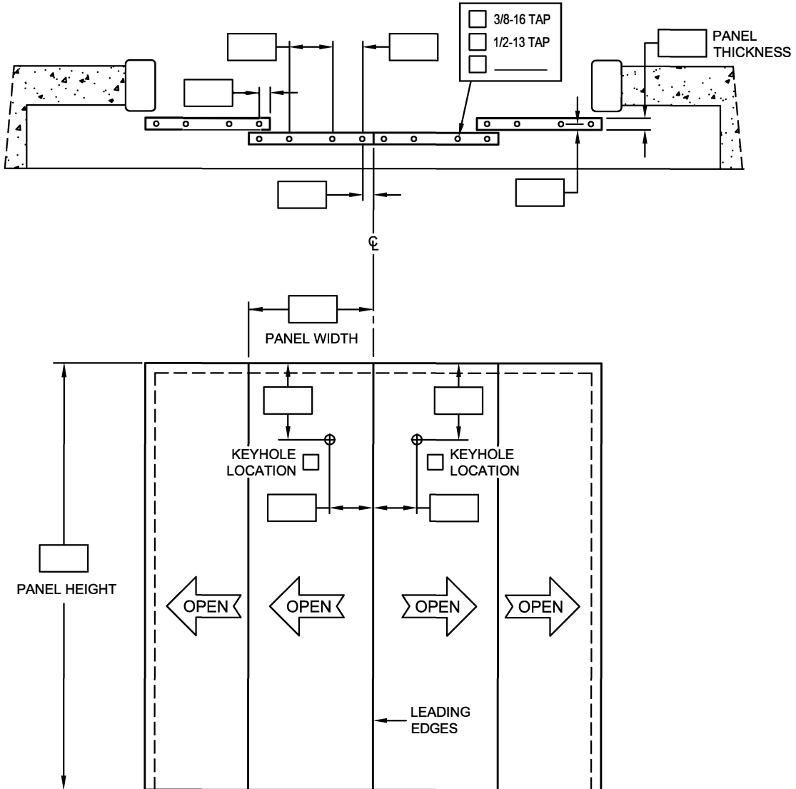
VIEWED FROM INSIDE HOISTWAY
