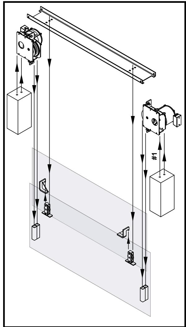
DOUBLE COUNTERWEIGHT
