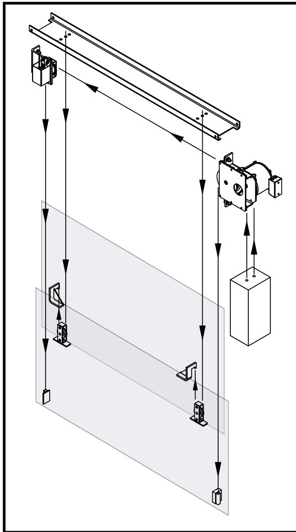
SINGLE COUNTERWEIGHT
